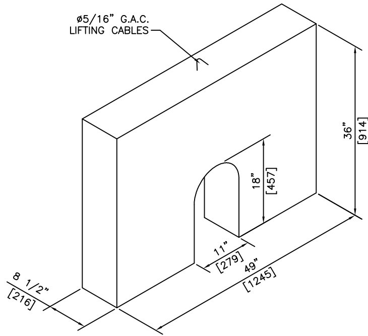
ISOMETRIC
