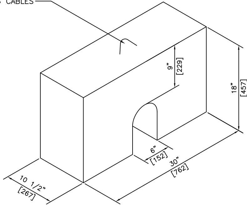
ISOMETRIC
