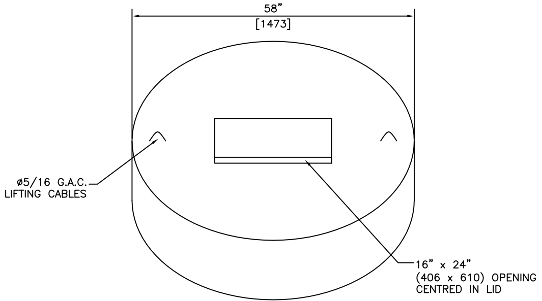
ISOMETRIC
