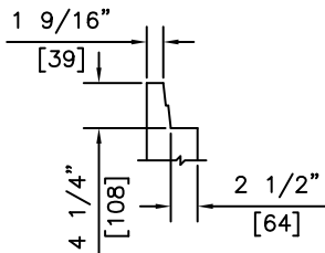
DETAIL
