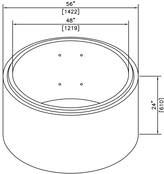
ISOMETRIC
