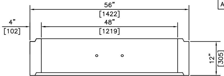
SECTION
