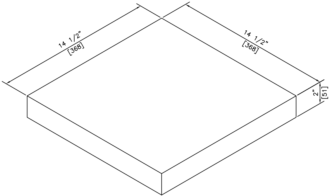
ISOMETRIC
