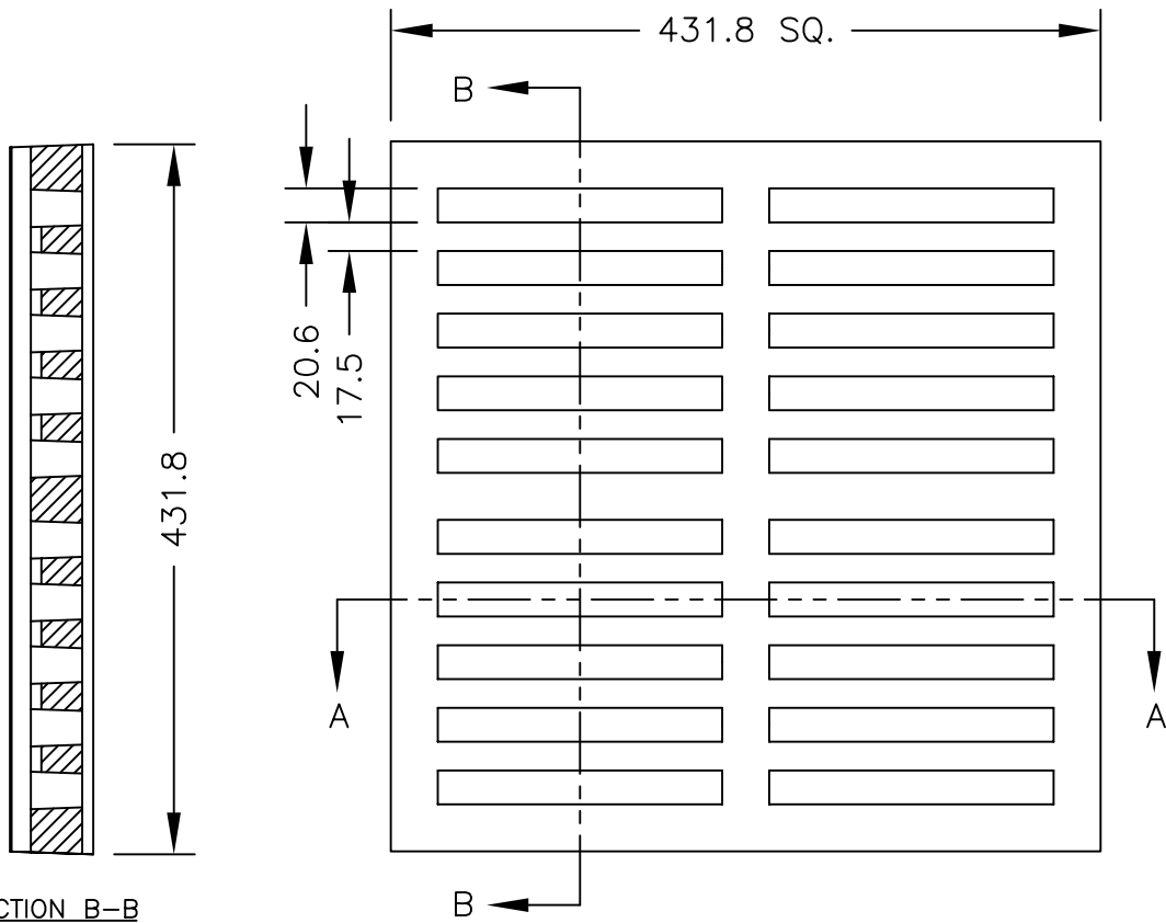
SECTION B-B
