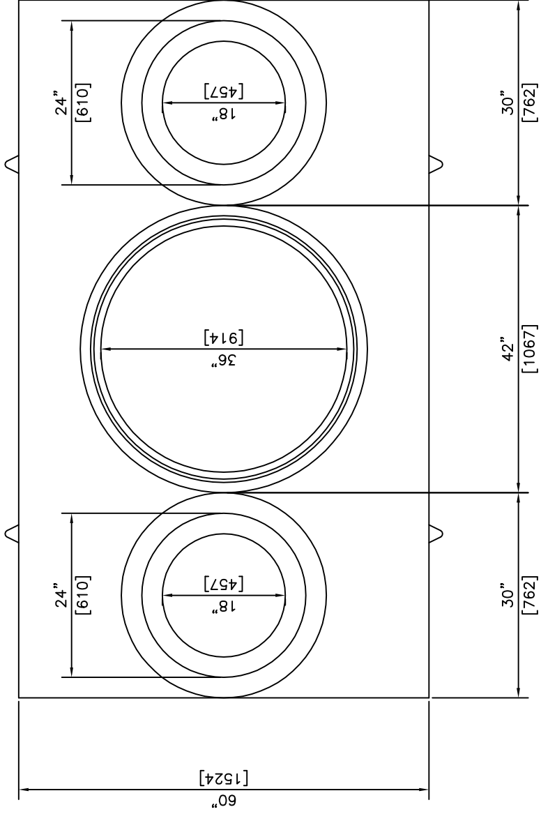
PLAN VIEW
